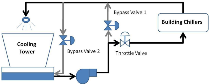
Figure 1: Simplified Schematic of Building Cooling System
