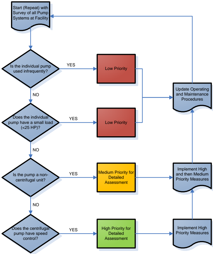
Figure 26: Pump Prioritization Flowchart
