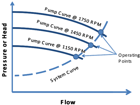
Figure 11: Centrifugal Pump Capacity as a Function of Pump Speed
